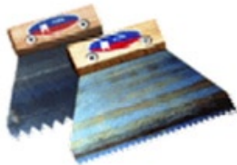
Adhesive scraper YORK® type 700(710) high carbon hardened steel, flexible blade, hard wood handle, riveted teeth 3(8)mm, size 140mm
